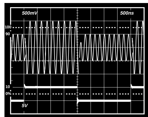
Figure 2. Channel Switching Characteristics for a 3:1 Mux
